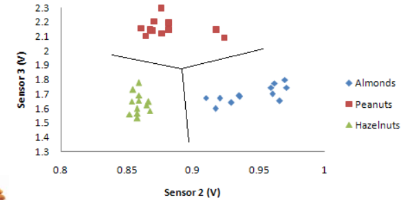
Sensor 2 vs. Sensor 3 Output (Cumulative)
