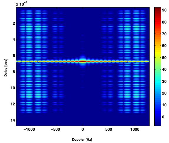
Fig. 1. Ambiguity function of a length- (N = 2^8) PTM pulse train of Golay complementary waveforms is free of range sidelobes along modest Doppler frequencies.
