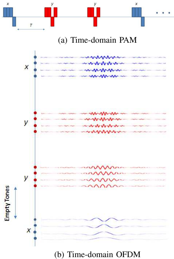
Fig. 2. Dual (PAM and OFDM) designs for sidelobe suppression. (a) Time-domain PAM (or frequency-domain OFDM) design for range sidelobe suppression. The pulse s(t) used in PAM is a square pulse. (b) Time-domain OFDM (or frequency-domain PAM) design for Doppler sidelobe suppression. Each OFDM subcarrier transmits a modulated sinc function a_m e^{-j m \omega_c t} S(t) . The empty tones correspond to the locations where a_m is zero. The Golay complementary sequences used in this example are \{x_\ell\} = \{1, 1, 1, -1\} and \{y_\ell\} = \{1, 1, -1, 1\} . Sequencing of x and y across time or frequency is performed according to the PTM sequence 01101001..., with 0 corresponding to x and 1 corresponding to y .
